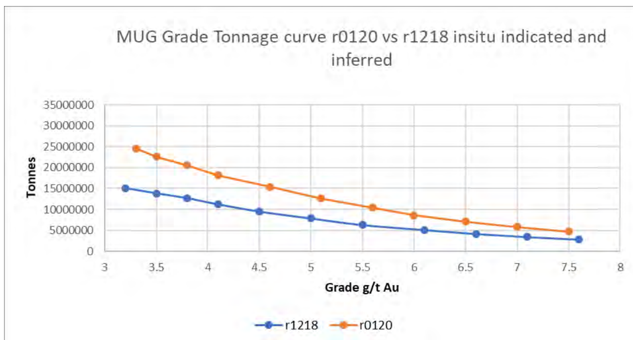
Figure 14-11: MUG Grade Tonnage Curve Comparing r0120 to r1218
