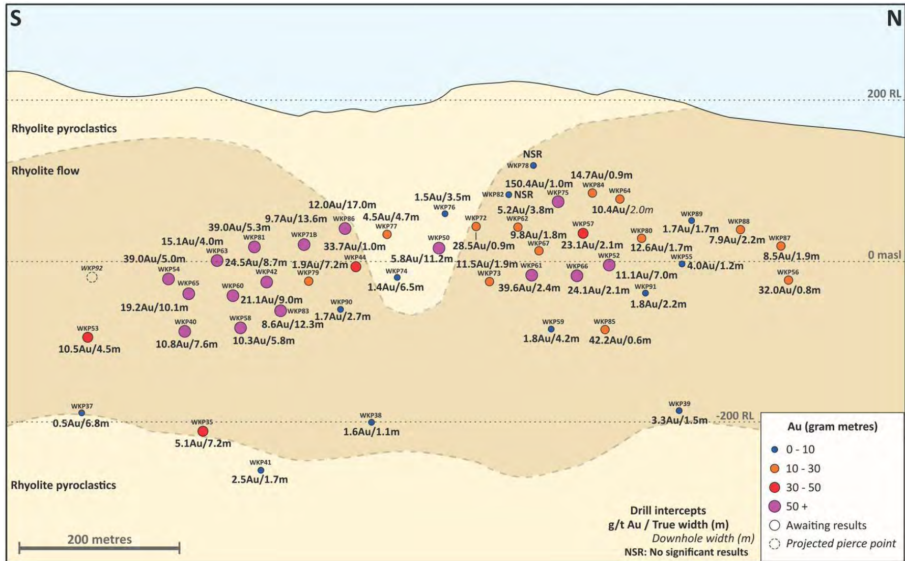
Figure 7-4: Simplified Long Section along the EG Vein at WKP (at Dec 2019).
