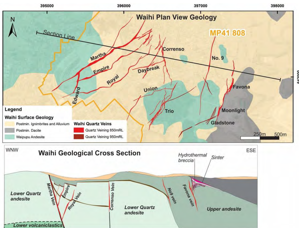
Figure 7-2: Geological Map and section across the Waihi area
