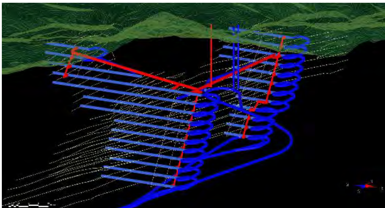
Figure 16-16: Primary Ventilation Circuit
