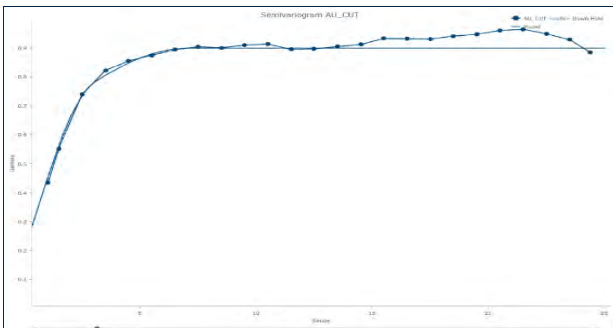
Figure 14-7: Omni directional Semi-variogram for the MUG diamond drilling data
