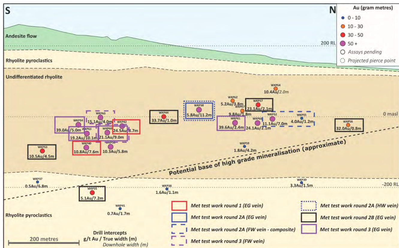
Figure 13-3: Long Section along the EG Vein at WKP
