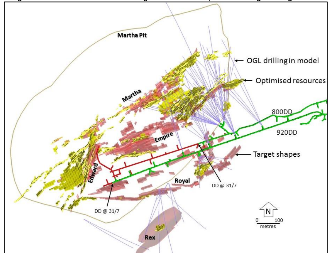
Figure 2.4: Plan View of Martha Underground Resources, recent drilling and target areas
