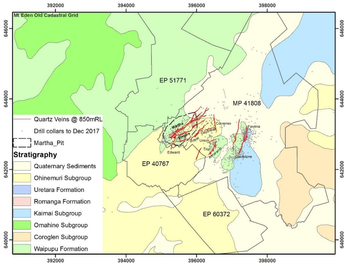
Figure 1-1: Project Geology Plan
