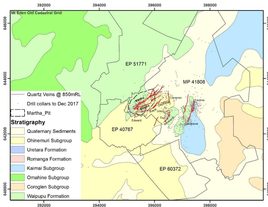
Figure 1-1: Project Geology Plan
