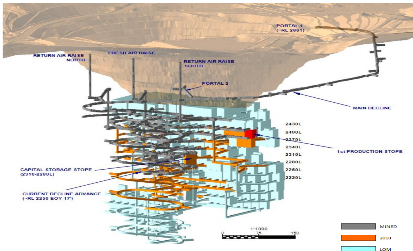
Figure 2 – Cross-section of Didipio Underground Design and Construction Phase
