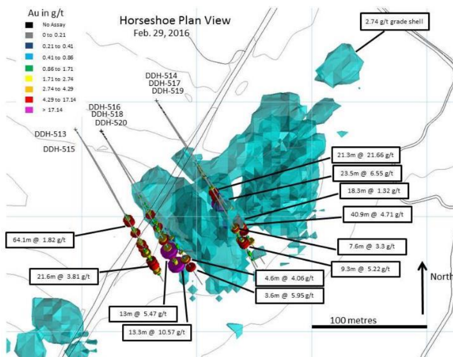
Figure 2 – Plan view of the Horseshoe deposit 2.74 g/t Au grade shell and recent drill results
