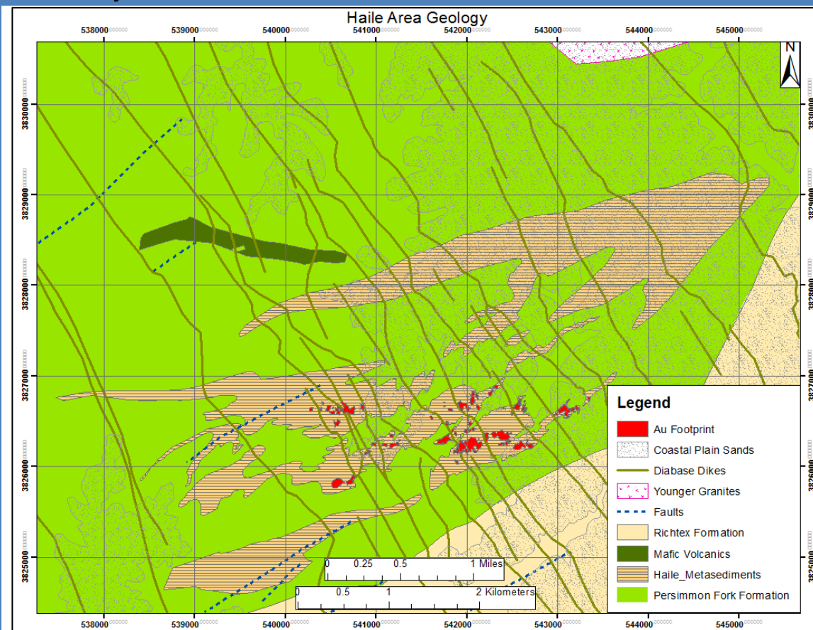
Schematic Geologic Map of Haile Mine area
