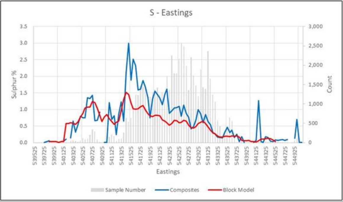
Swath Plot with Mean Composite Carbon Grade vs HA0520OLM Block Values
