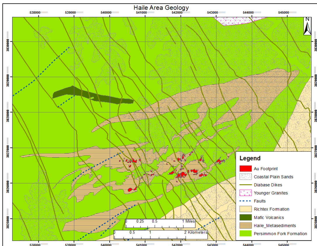
Figure 3: Schematic Geologic Map of Haile Mine area
