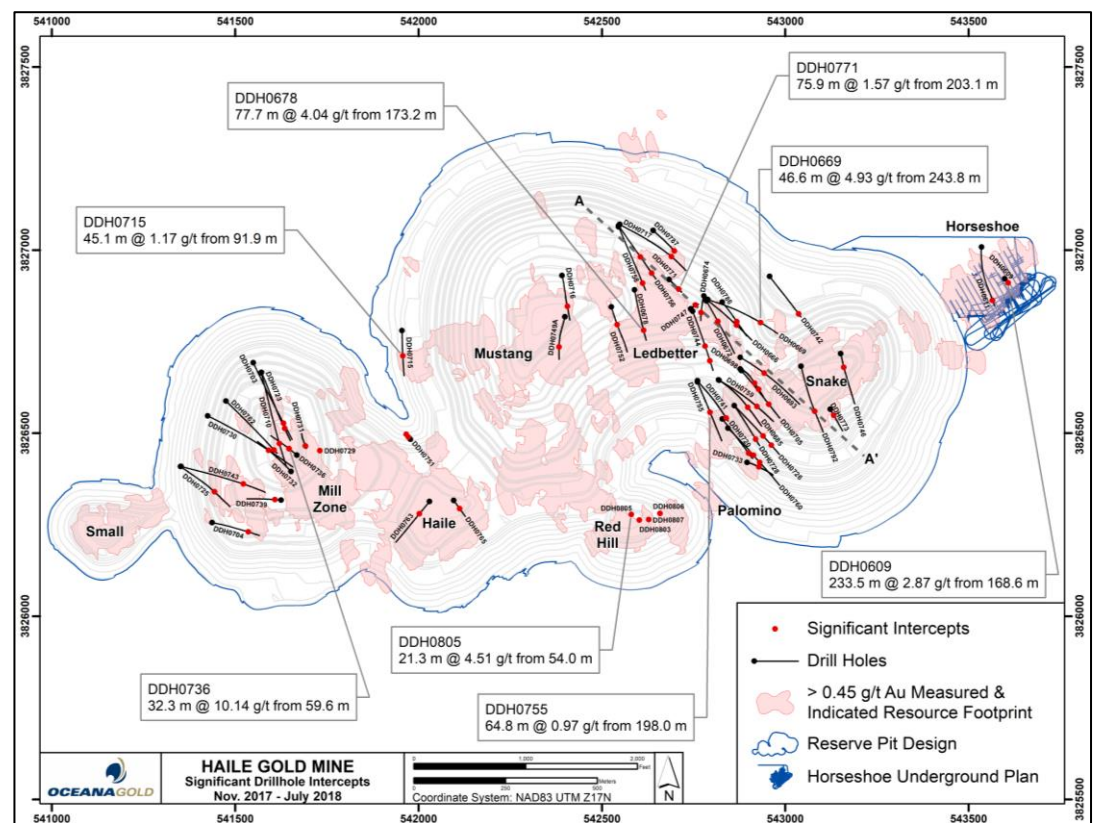
Figure 4: Plan map of Haile gold mineralisation 2018 drilling
