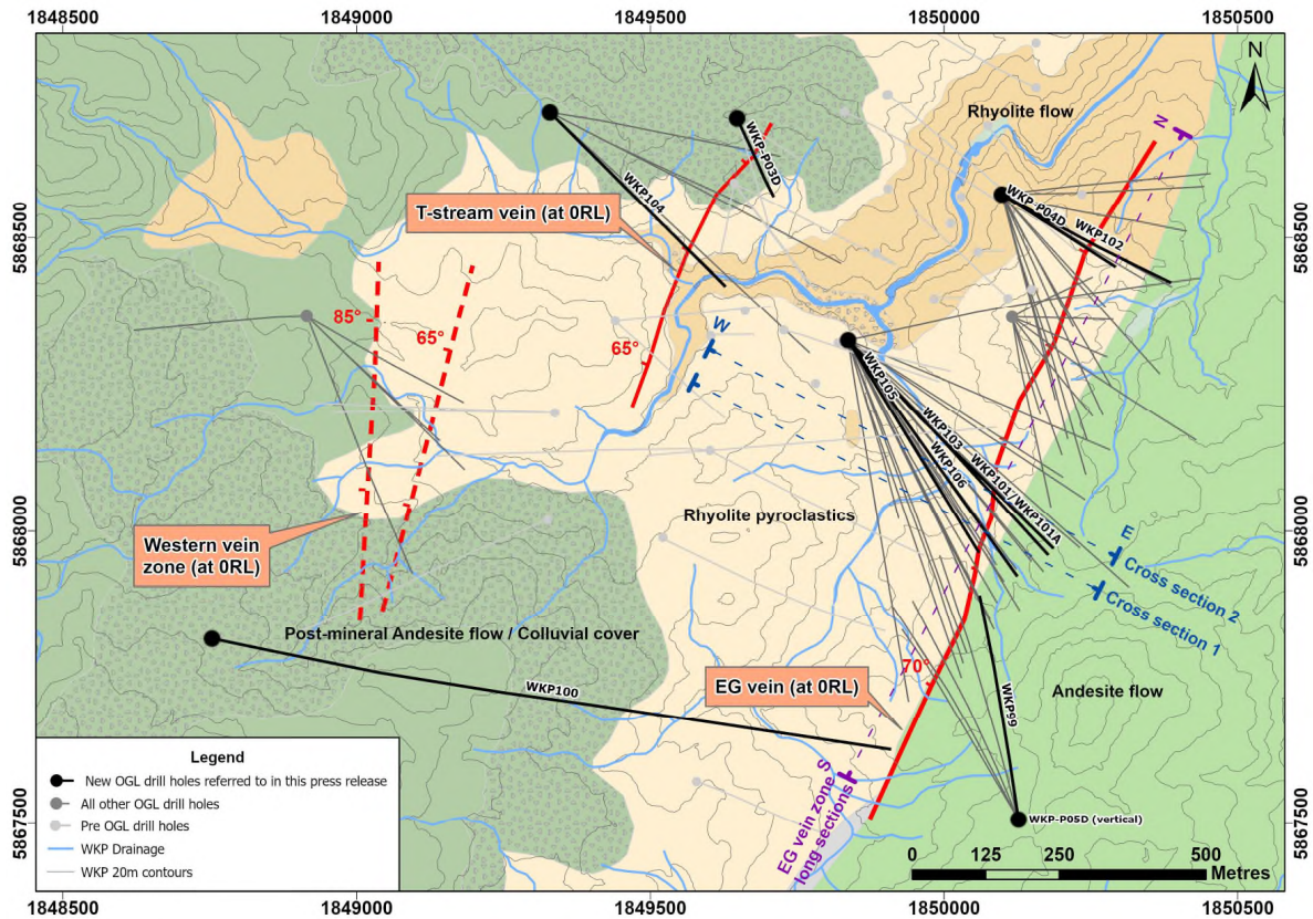
Figure 1: Plan View of Geology, Drill traces and Distribution of 3 Main Veins at WKP.
