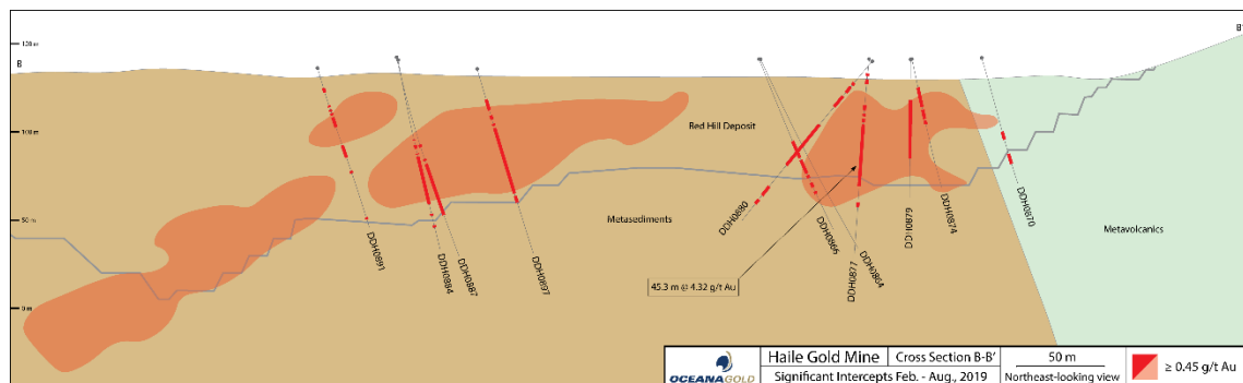
Figure 6: Long section B-B' through Red Hill deposit, looking northwest
