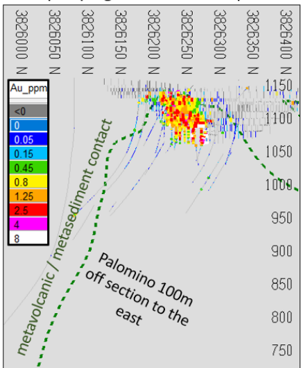
Figure 6: Cross-Section of Red Hill Grade Control Drilling (left) and Palomino Resource Drilling (right), relative to the Metavolcanic / Metasediment contact
