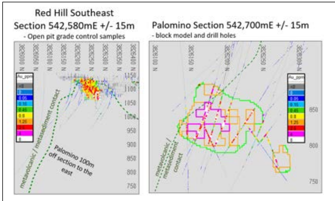
Figure 14-32 Cross-Section of Red Hill Grade Control Drilling and Palomino Resource Drilling
