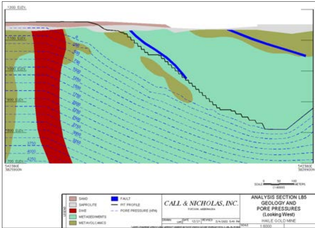
Figure 16-3: Example of Steady State Pore Pressure Estimates: Cross-Section LB5 for the South Wall of the Ledbetter Pit
