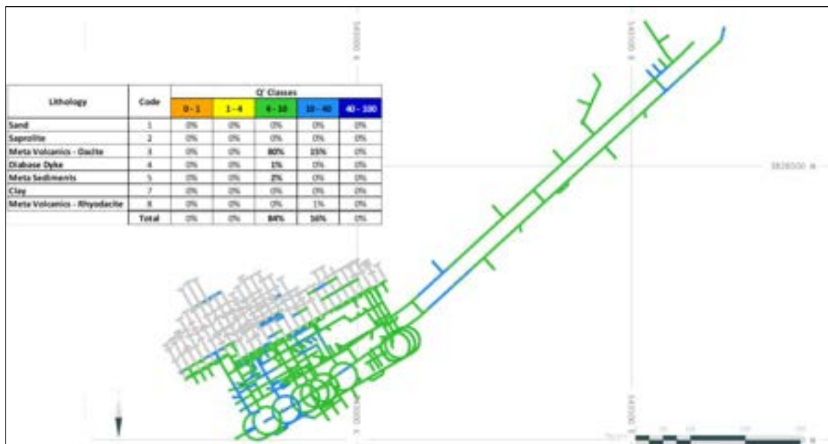
Figure 16-29: Rock Quality On Permanent Development - Palomino
