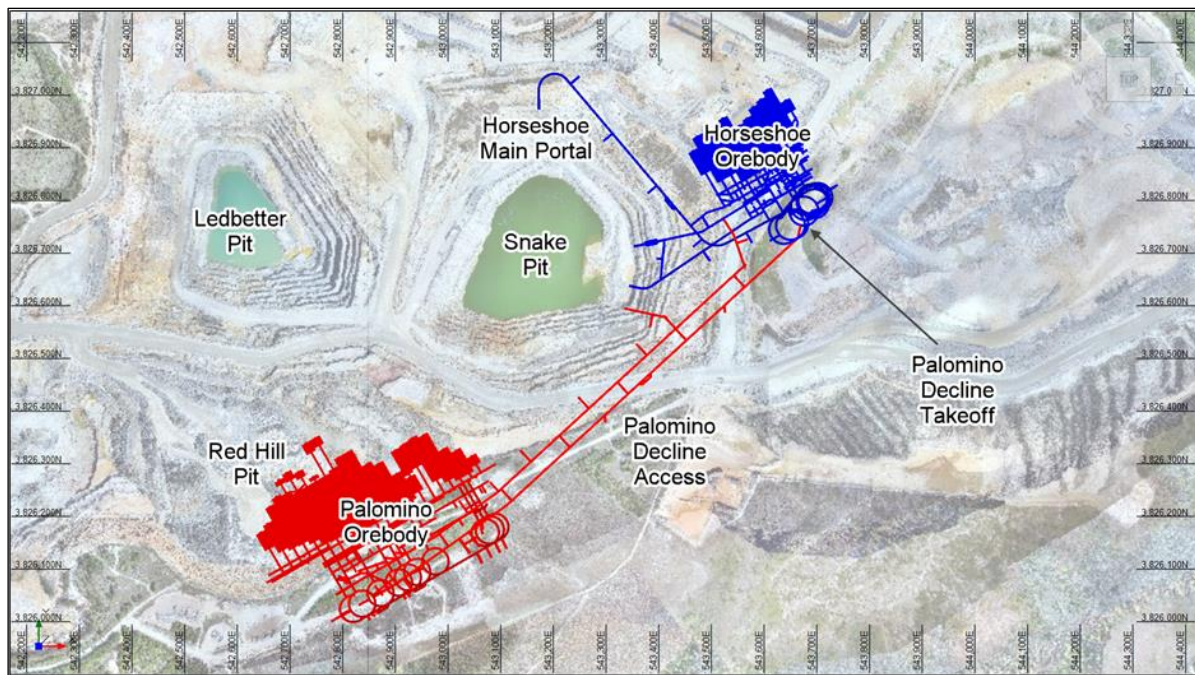
Figure 15-1: General Site Layout and Location of the UG Reserve Area (in blue and red)
