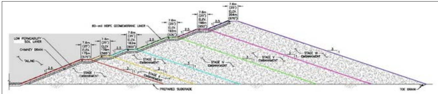
Figure 18-2: Tailing Storage Facility Typical Section
