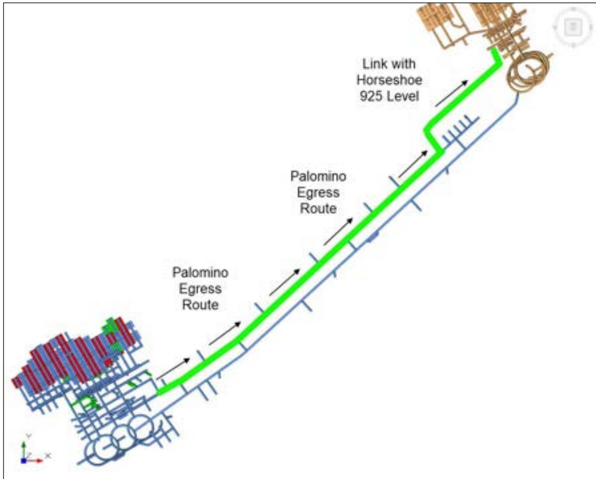
Figure 16-47: Palomino Egress via Horseshoe - Plan View
