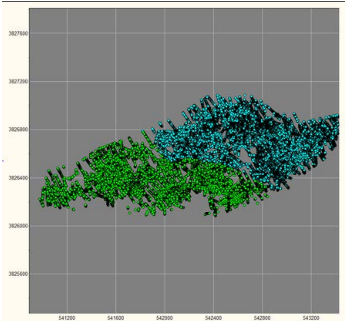
Figure 14-1: Estimation Domains
