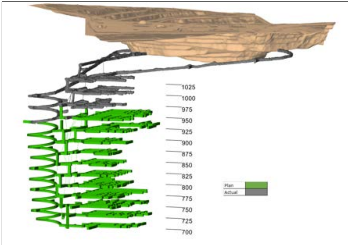
Figure 16-36: Horseshoe Development Asbuilt and Plan
