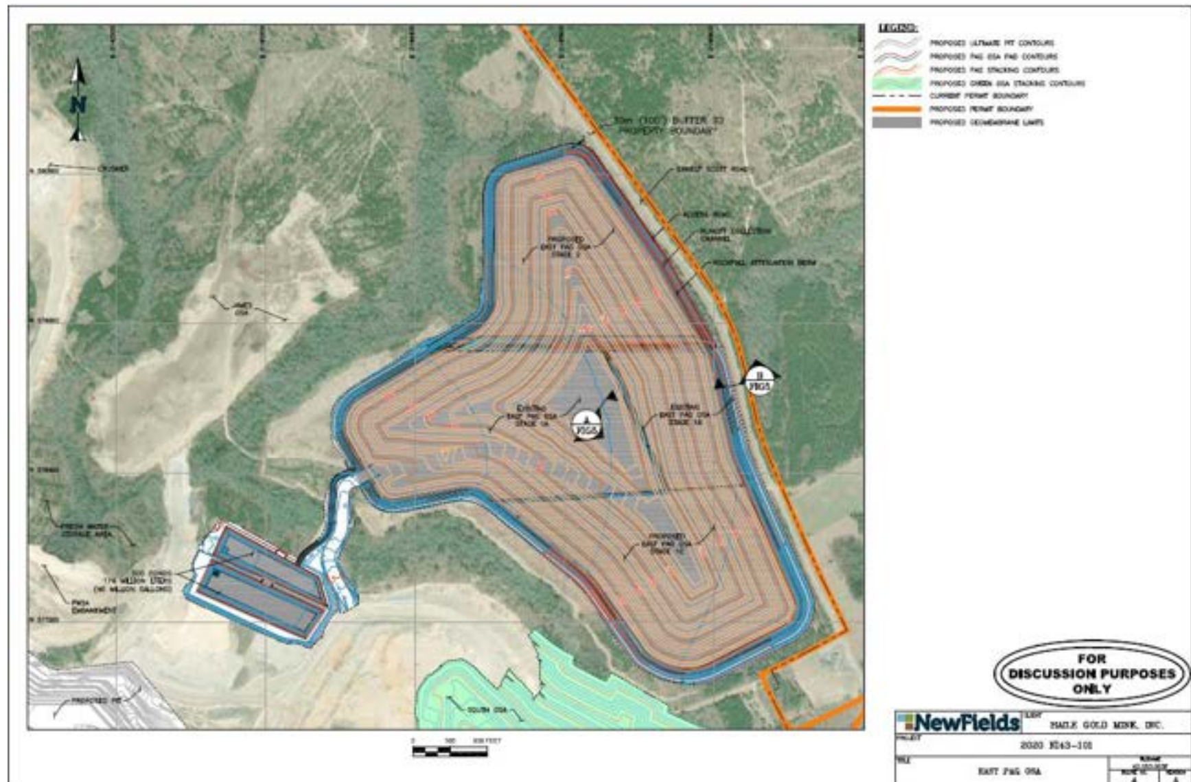
Figure 18-5: East PAG Overburden Storage Area Expansion
