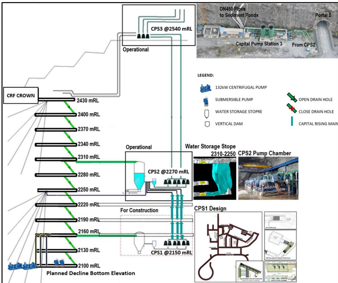
Figure 16-48: Didipio Pump System Schematic
