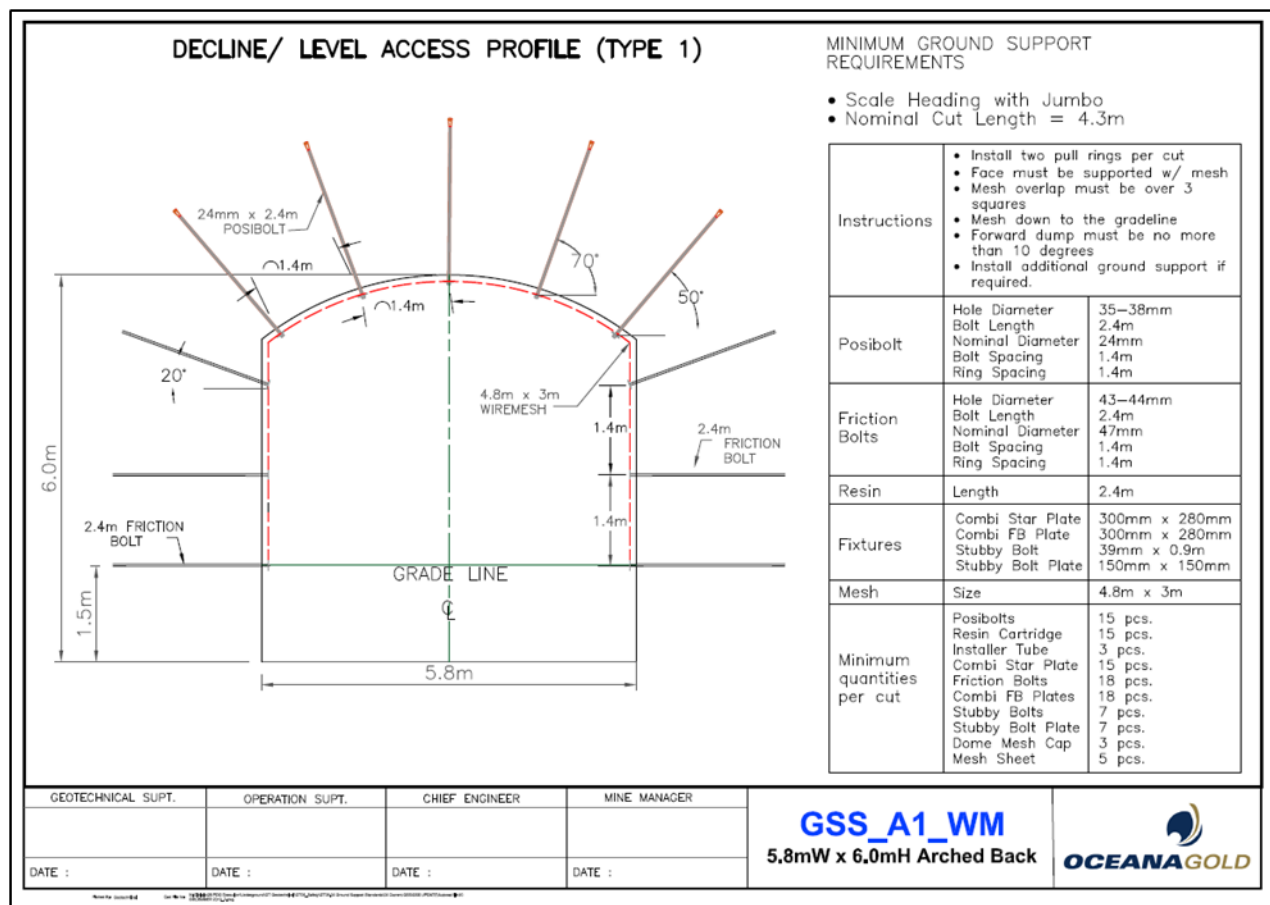
Figure 16-14: Decline (A1) Approved Ground Support Standard
