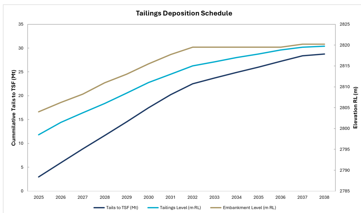
Figure 18-2: LoM Storage Requirements and Scheduled TSF Development
