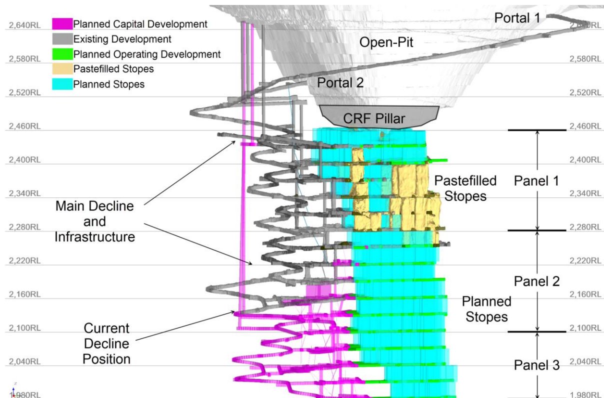
Figure 16-1: Didipio Underground – Oblique view Looking North- West
