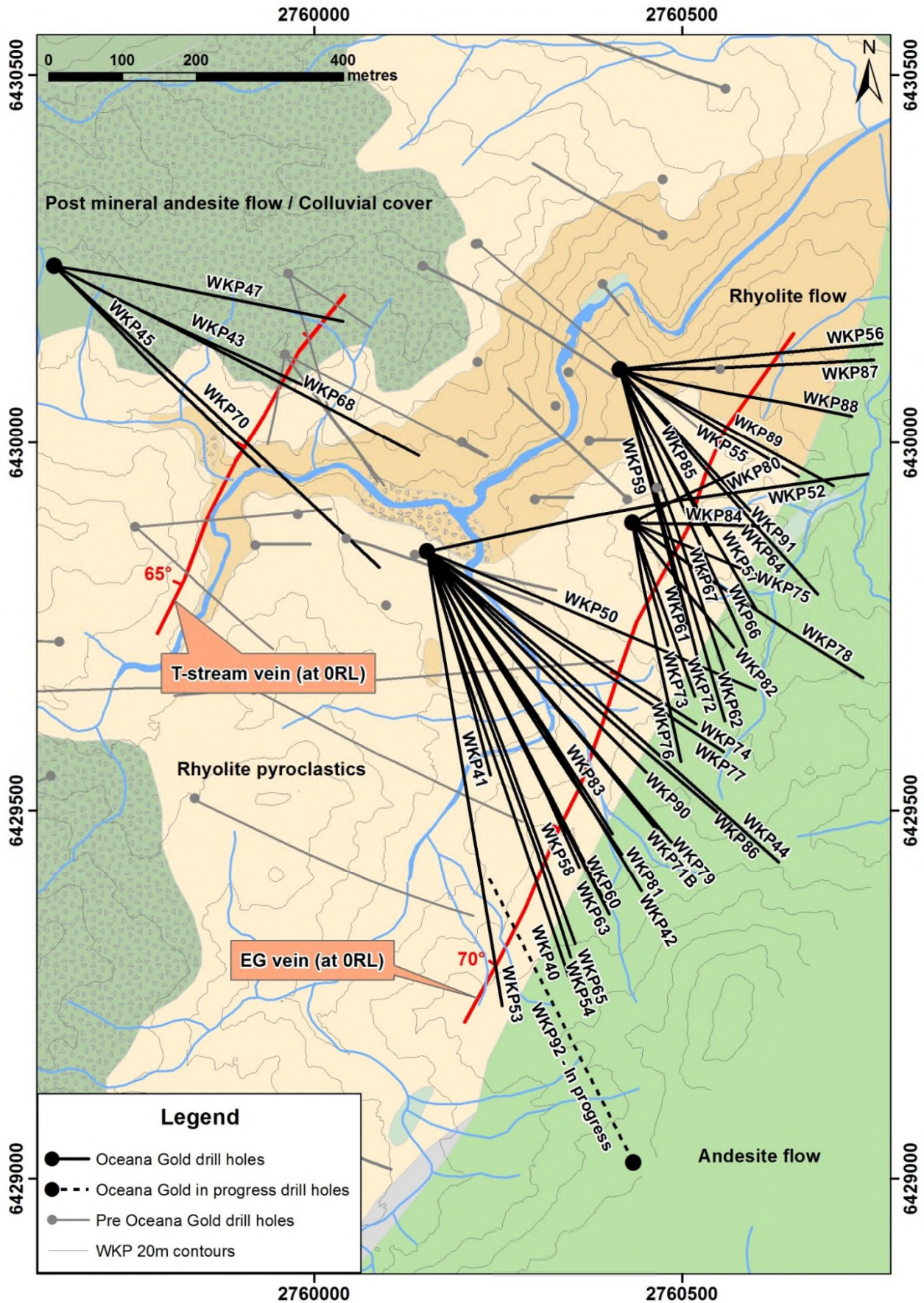
Figure 1: Map showing the surface geology and drilling along the East Graben (EG) vein, WKP (OceanaGold drillholes 2017 to Dec 2019)
